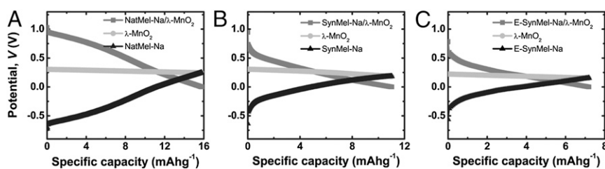
Fig. 4. Potential profiles of full cells are shown using Na + -loaded melanin anodes and λ-MnO 2 cathodes under discharge rates of -10 μA. Discharges were measured in 1 M Na 2 SO 4 with Pt counter and reference electrodes. Specific charge storage capacities based on active anode masses were 16.1 ± 0.8, 12.4 ± 1.2, and 7.9 ± 1.4 mA h g -1 for (A) NatMel-Na, (B) SynMel-Na, and (C) E-SynMel-Na, respectively ( n = 5).
